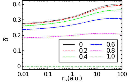
FIG. 15. Relative energy deviations \delta^P from QMC results for different polarizations \xi \in [0, 1] .
