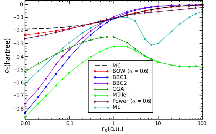
FIG. 17. Comparison of the exact QMC correlation energy of the 2D HEG in the Attacalite parametrization [74] (black curve) with the predictions of the BOW functional (red curve) and various other RDMFT XC functionals.
